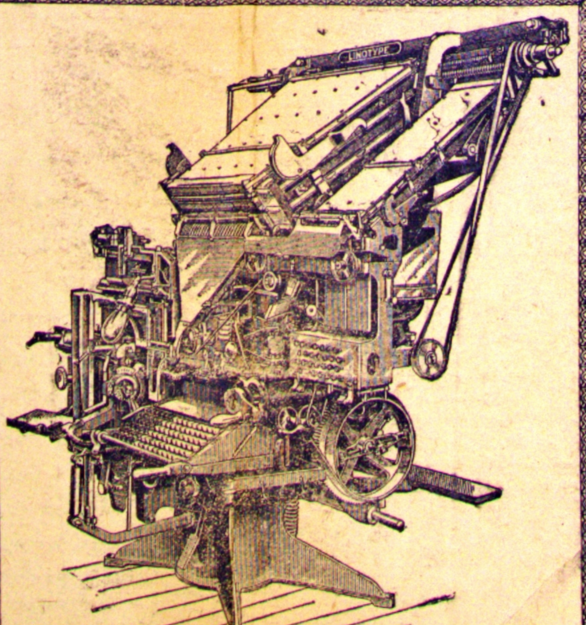
Three-Magazine Model Fourteen Linotype
