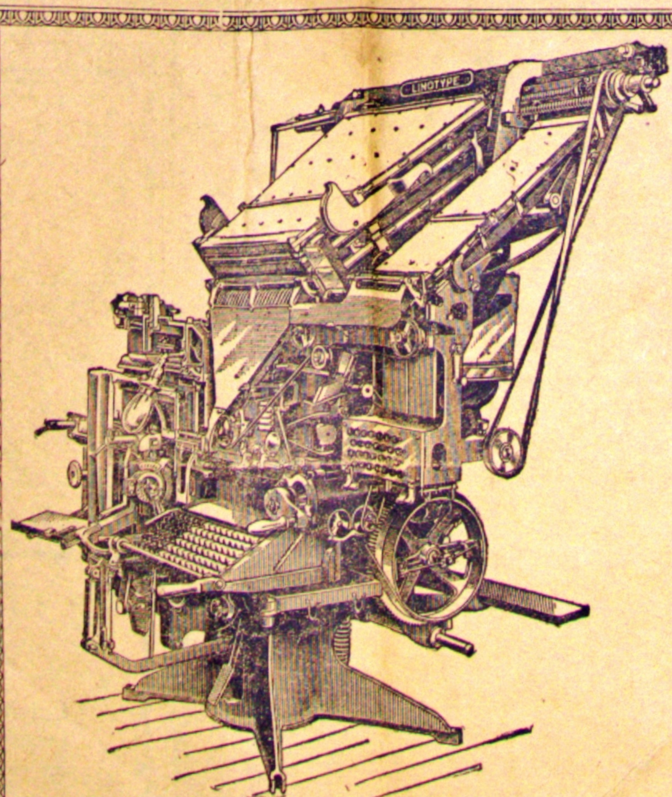
Three-Magazine Model Fourteen Linotype
